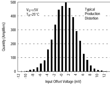
EL5410C Input Offset Voltage Distribution
